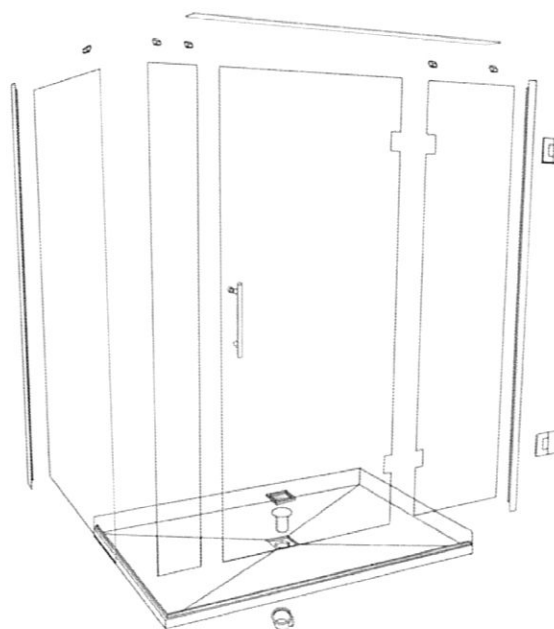
Illustrated profile of artisan tile shower system: rectangular shower base, waste & screens.
